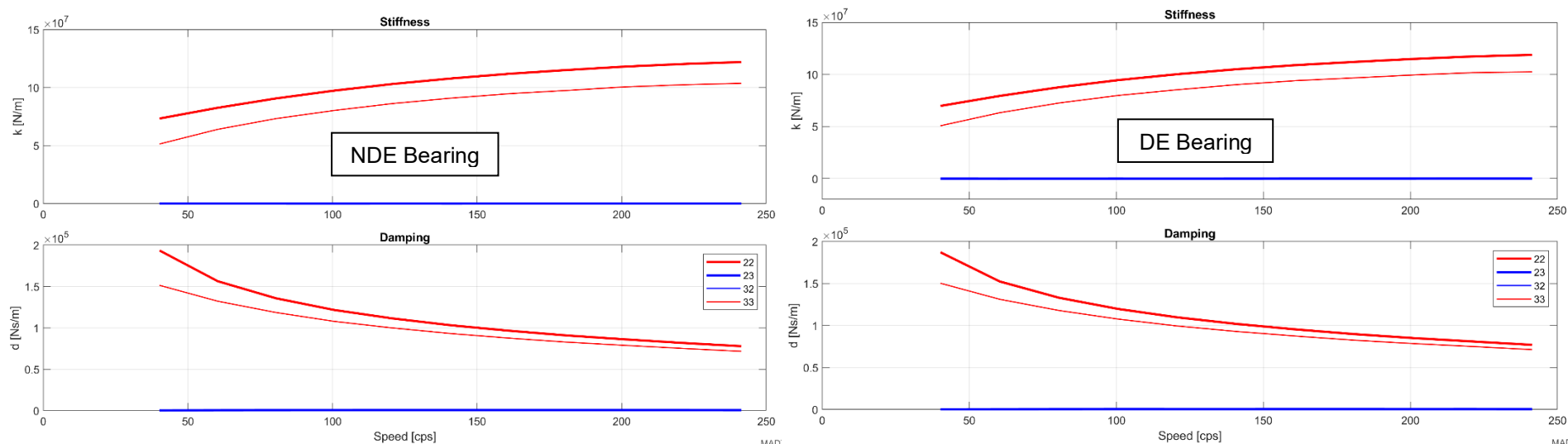
Fig. 3.2: Rotordynamic stiffness and damping coefficients for the static loads without seal influence
