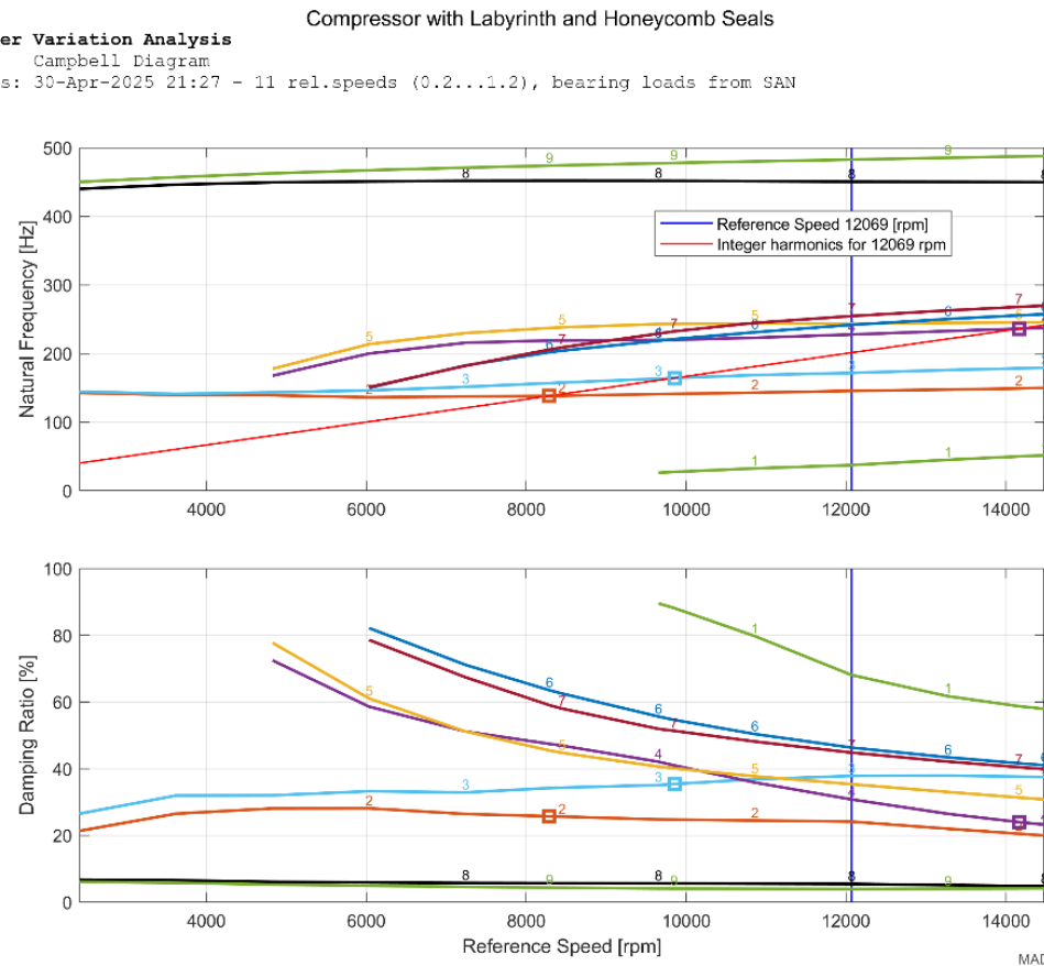
Fig. 3.8: Campbell diagram with seals
