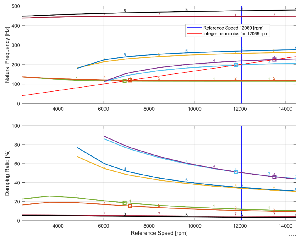
Fig. 3.3: Campbell diagram without seals with mode shapes in critical speeds (no load condition)
