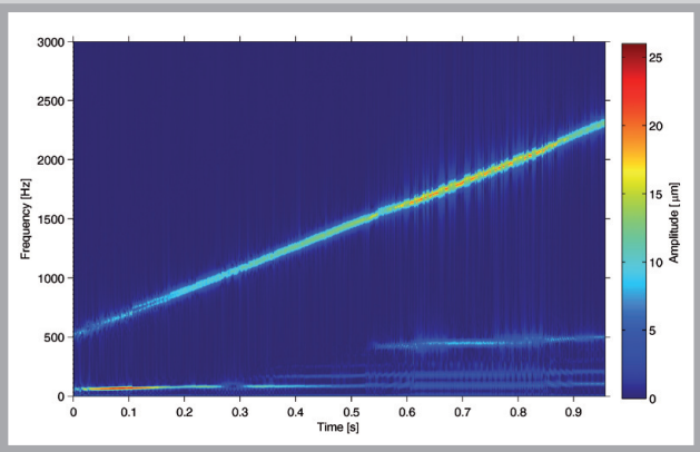
Spectrum of the non-linear transient run up of a turbocharger
