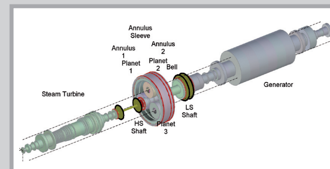
Model of a steam turbine generator train with planetary gear
