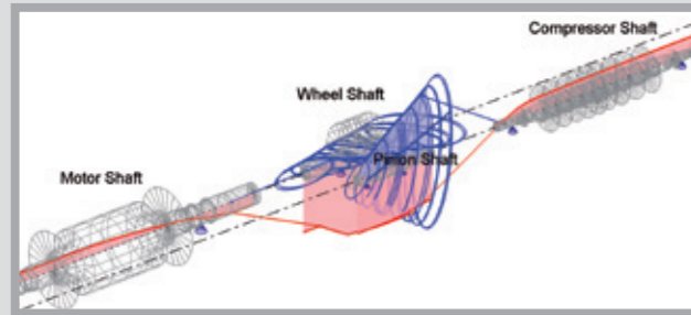
Coupled lateral torsional vibration mode
