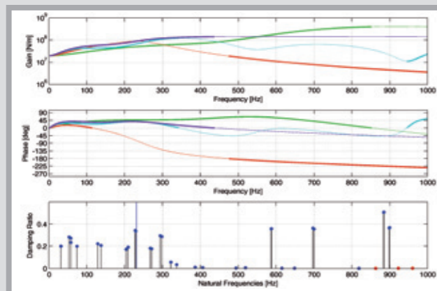
Magnetic bearing transfer functions with eigenvalues for stability check
