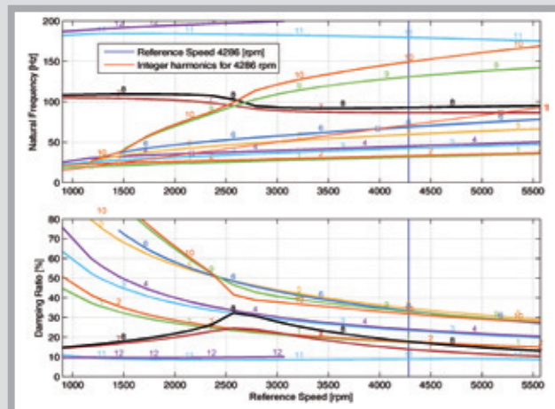
Campbell diagram of system with inner and outer rotor
