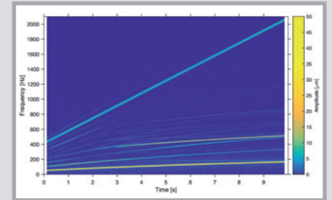
Spectrum of the nonlinear transient run up of a turbocharger
