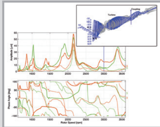
Resonance curve of casing vibrations at support with shape at 3400 rpm
