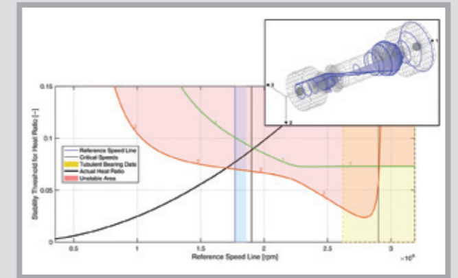
Hot spot stability chart (Morton effect) with shape at lowest threshold
