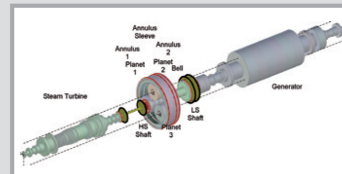
Model of a steam turbine generator train with planetary gear
