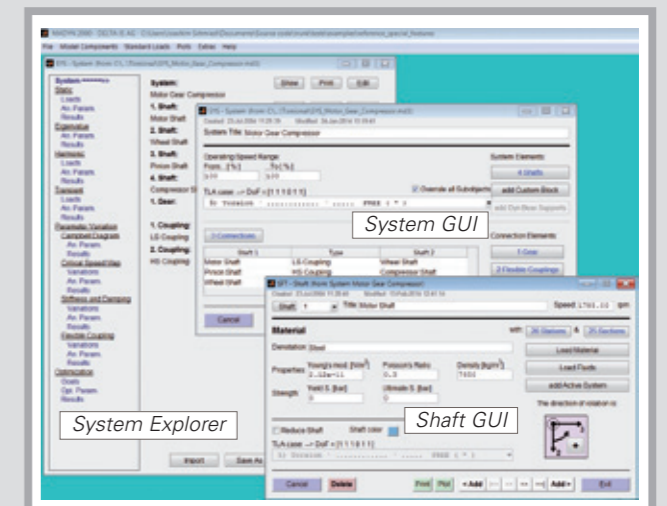
System explorer with graphical user interfaces
