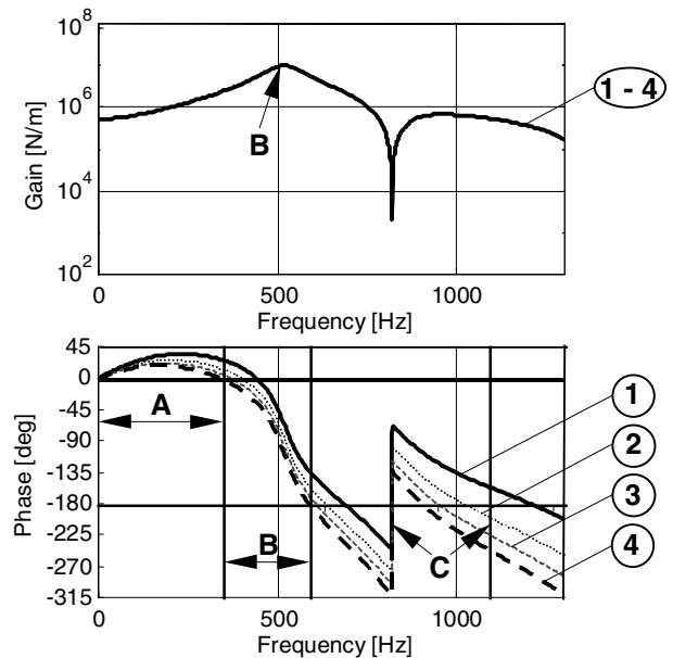
Fig. 3 Bearing Transfer Function of the TMP
