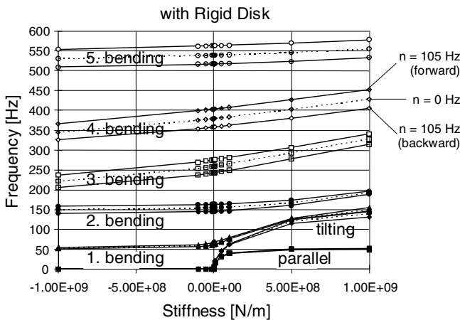
Fig. 4 Natural Frequencies of the Modes vs. Bearing Stiffness and Speed (rigid fixed disk)
