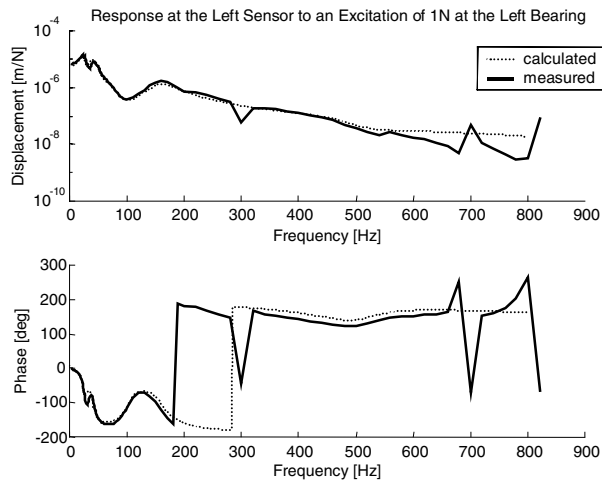
Fig. 8 Measured and Calculated Responses at 300 cps
