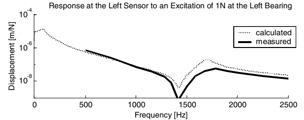
Fig. 7 Measured and Calculated Responses at Standstill
