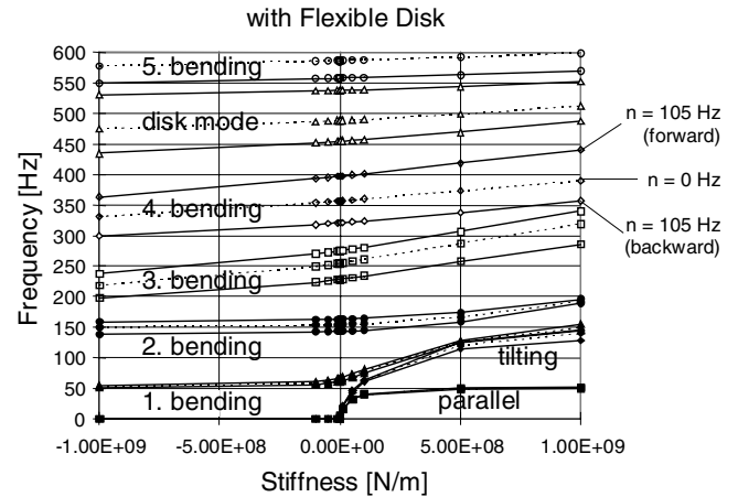
Fig. 5 Natural Frequencies of the Modes vs. Bearing Stiffness and Speed (flexible fixed disk)
