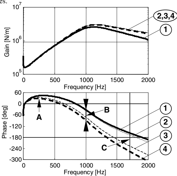
Fig. 1 Bearing Transfer Function of the High Speed Rotor
