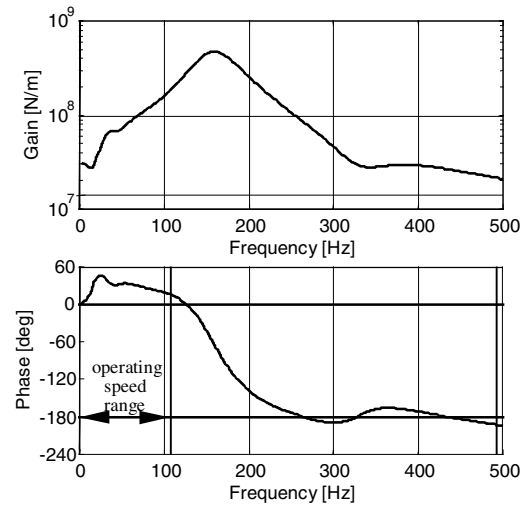
Fig. 6 Bearing Transfer Function of the Large Industrial Centrifugal Compressor
