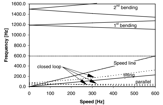
Fig. 2 Natural Frequencies of the Modes vs. Speed for the Free and Supported Rotor
